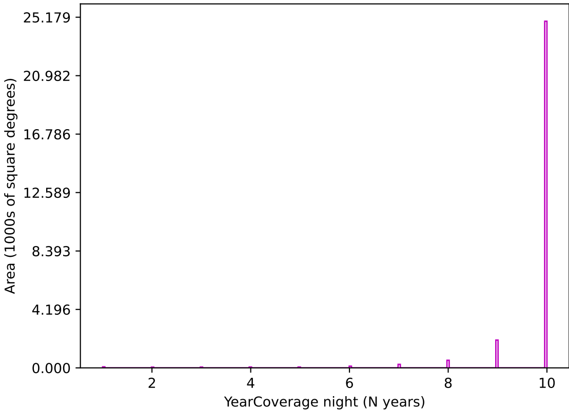
ddf_acor_sf15_lsf20_lsr20_v3.4_10yrs z band: YearCoverage night
