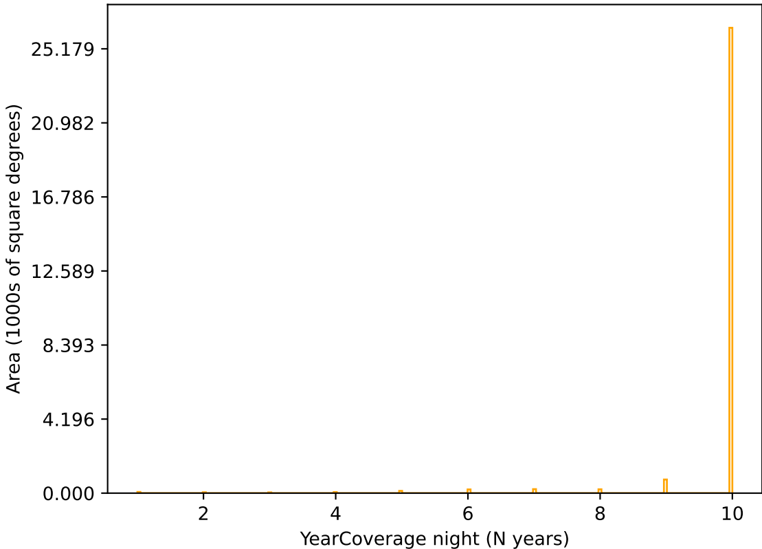
ddf_acor_sf15_lsf20_lsr20_v3.4_10yrs r band: YearCoverage night
