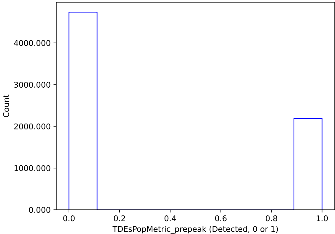
ddf_acor_sf15_lsf20_lsr20_v3.4_10yrs : TDEsPopMetric_prepeak
