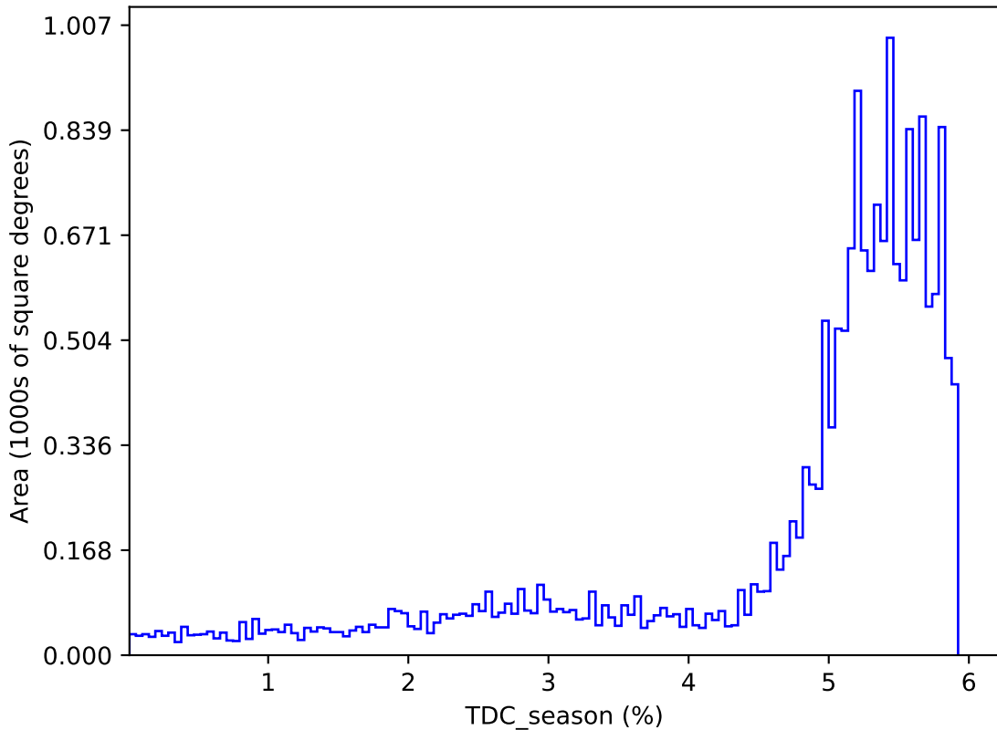
ddf_acor_sf15_lsf20_lsr20_v3.4_10yrs : TDC_season
