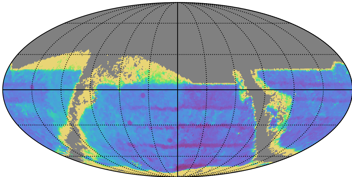
ddf_acor_sf15_lsf20_lsr20_v3.4_10yrs : TDC_accuracy
