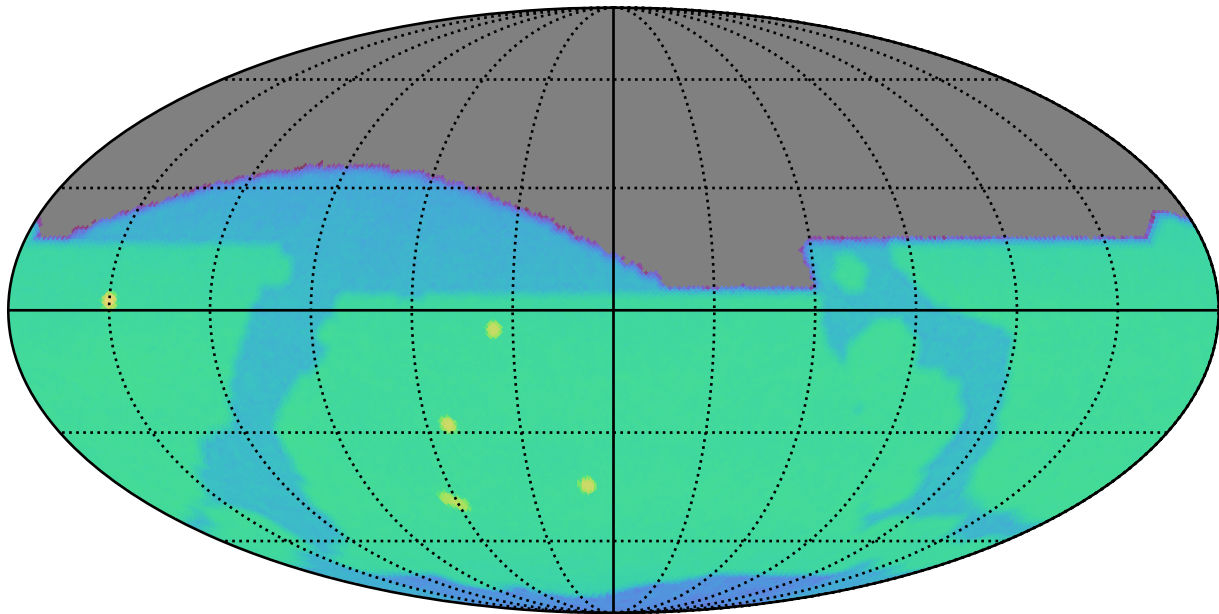
ddf_acor_sf15_lsf20_lsr20_v3.4_10yrs i: SurfaceBrightLimit
