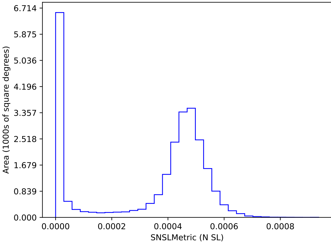
ddf_acor_sf15_lsf20_lsr20_v3.4_10yrs : SNSLMetric
