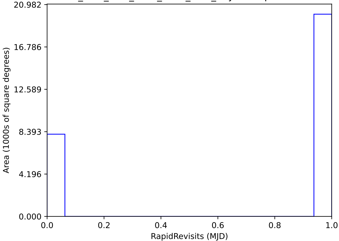
ddf_acor_sf15_lsf20_lsr20_v3.4_10yrs : RapidRevisits
