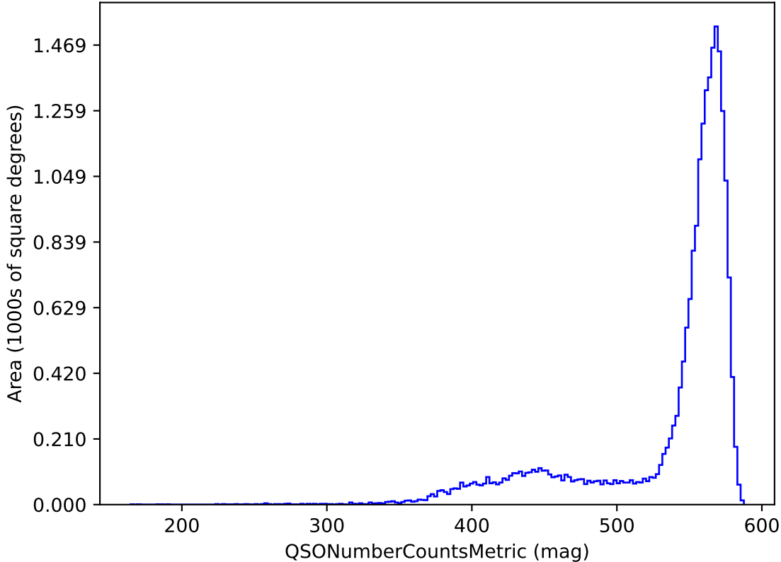
ddf_acor_sf15_lsf20_lsr20_v3.4_10yrs y band and non-DD: QSONumberCountsMetric
