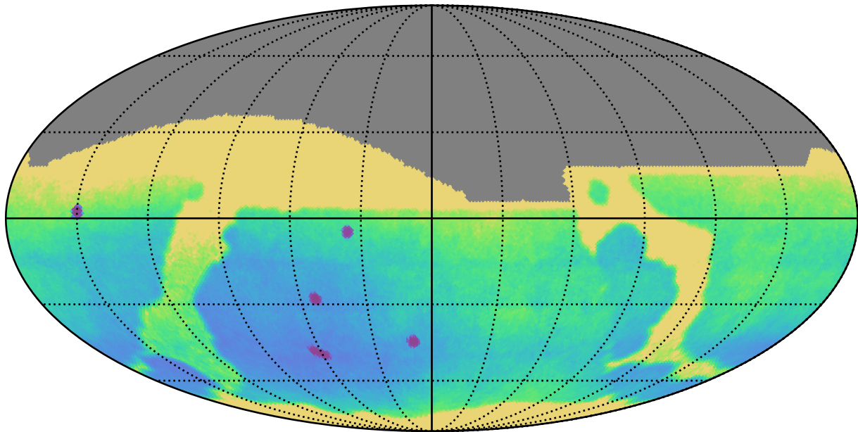
ddf_acor_sf15_lsf20_lsr20_v3.4_10yrs : Parallax Uncert @ 24.0
