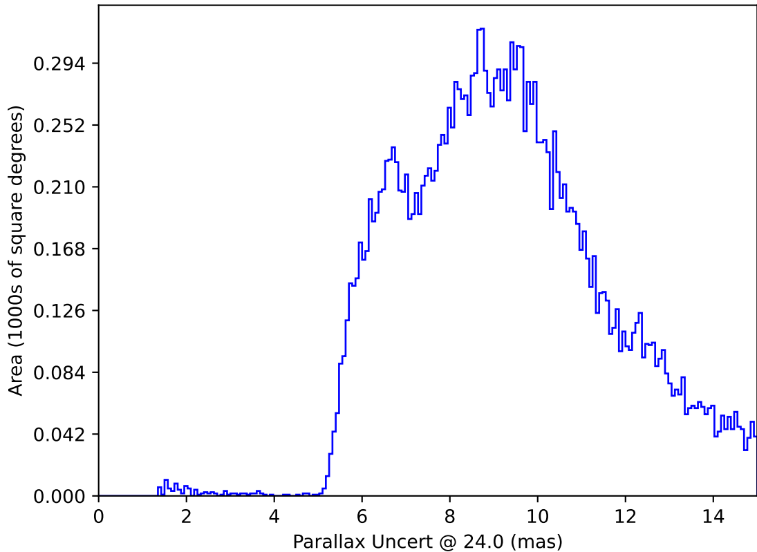
ddf_acor_sf15_lsf20_lsr20_v3.4_10yrs : Parallax Uncert @ 24.0
