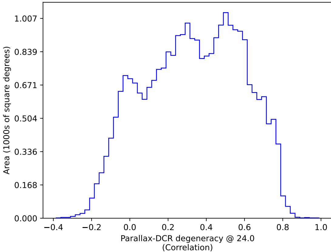
ddf_acor_sf15_ls20_lsr20_v3.4_10yrs : Parallax-DCR degeneracy @ 24.0
