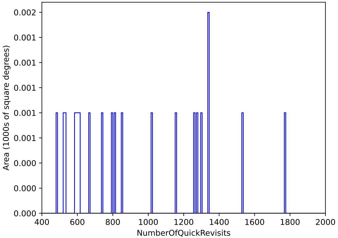
ddf_acor_sf15_lsf20_lsr20_v3.4_10yrs : NumberOfQuickRevisits
