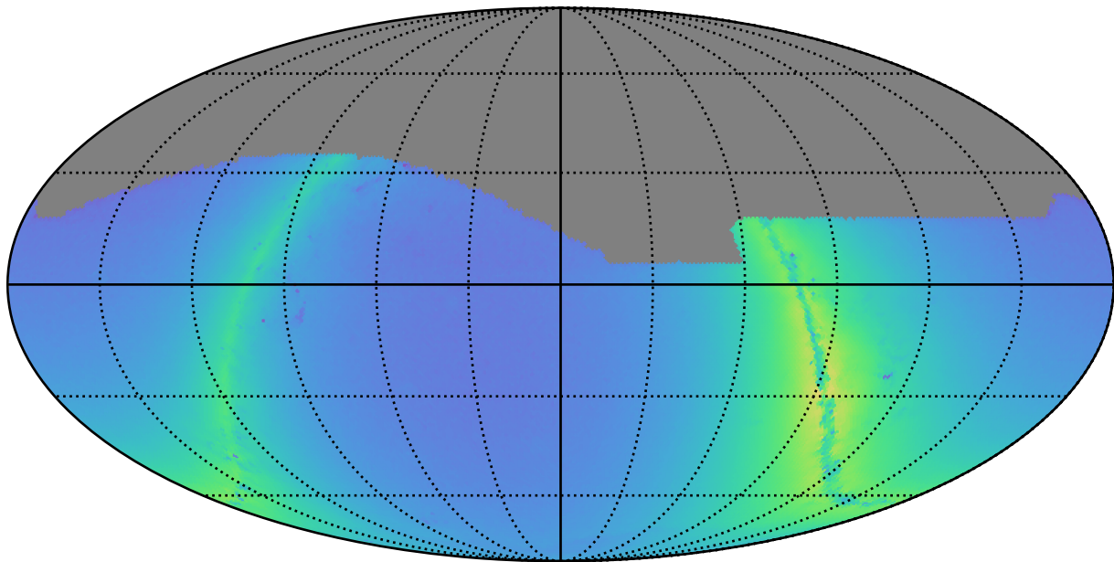
ddf_acor_sf15_lsf20_lsr20_v3.4_10yrs r: Nstars_no_crowding
