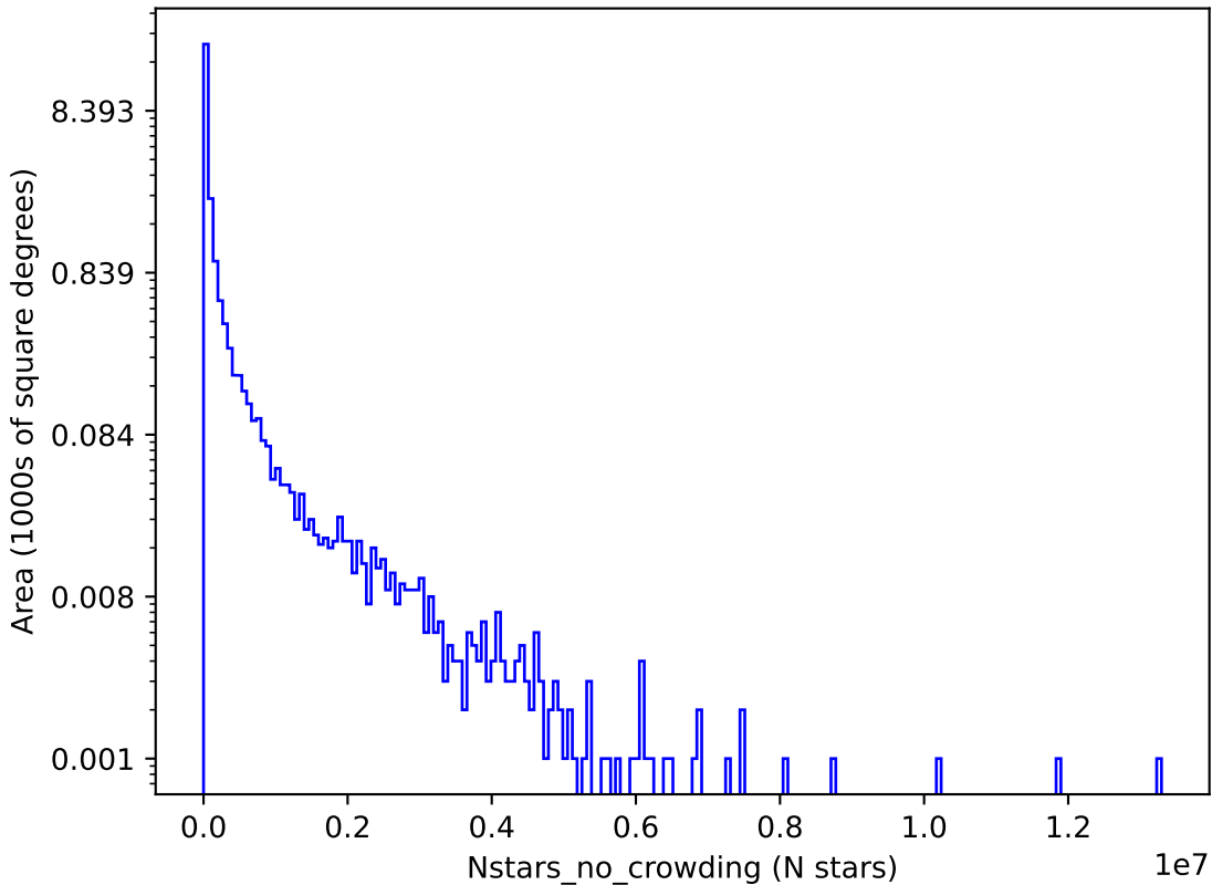
ddf_acor_sf15_lsf20_lsr20_v3.4_10yrs g: Nstars_no_crowding
