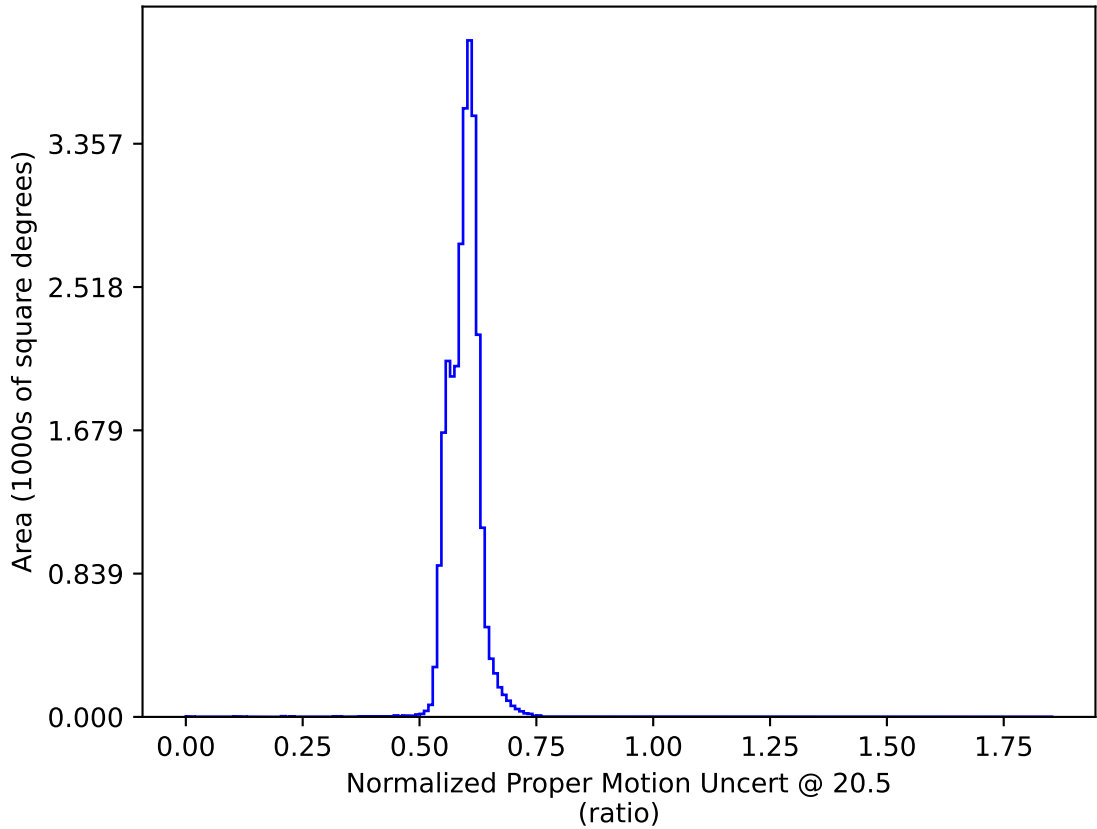
ddf_acor_sf15_lsf20_lsr20_v3.4_10yrs : Normalized Proper Motion Uncert @ 20.5
