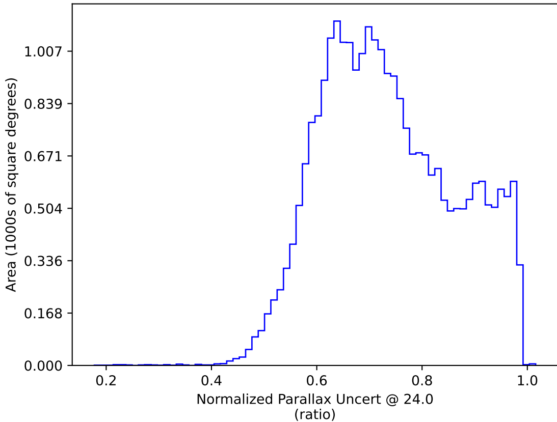
ddf_acor_sf15_lsf20_lsr20_v3.4_10yrs : Normalized Parallax Uncert @ 24.0
