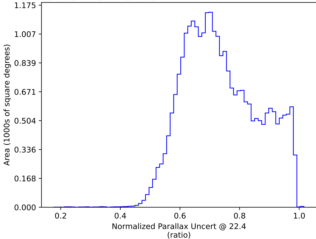
ddf_acor_sf15_lsf20_lsr20_v3.4_10yrs : Normalized Parallax Uncert @ 22.4
