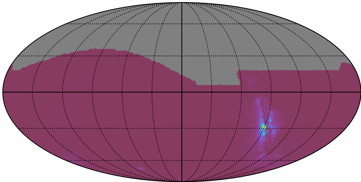
ddf_acor_sf15_lsf20_lsr20_v3.4_10yrs : NlcPoints
