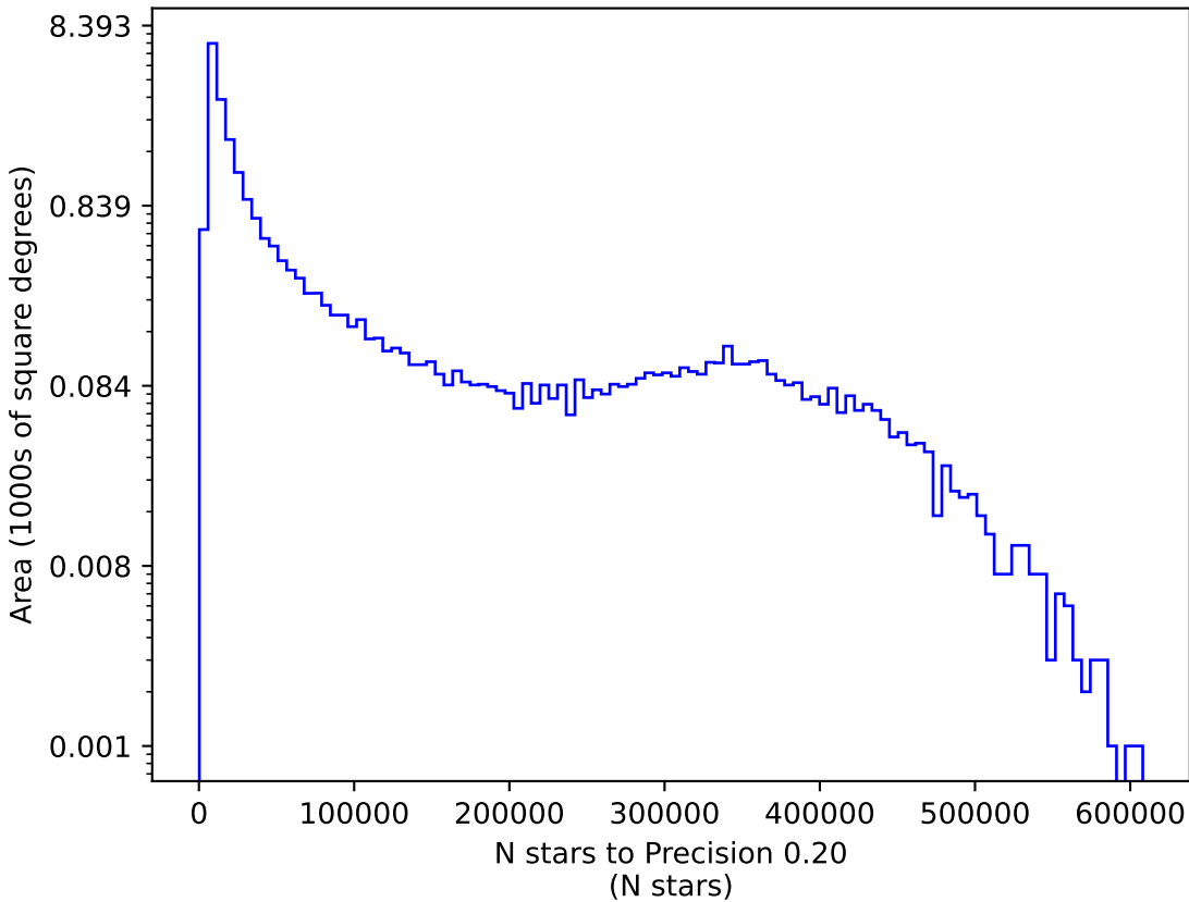
ddf_acor_sf15_lsf20_lsr20_v3.4_10yrs y: N stars to Precision 0.20
