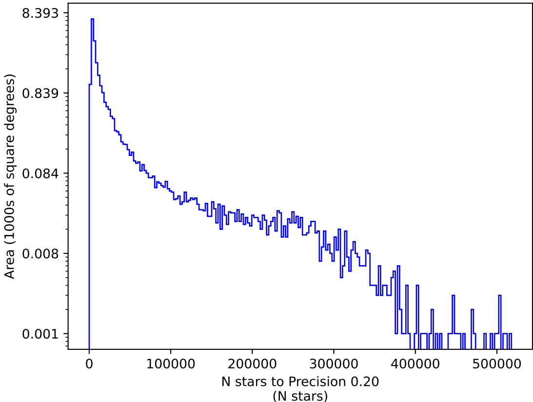
ddf_acor_sf15_lsf20_lsr20_v3.4_10yrs u: N stars to Precision 0.20
