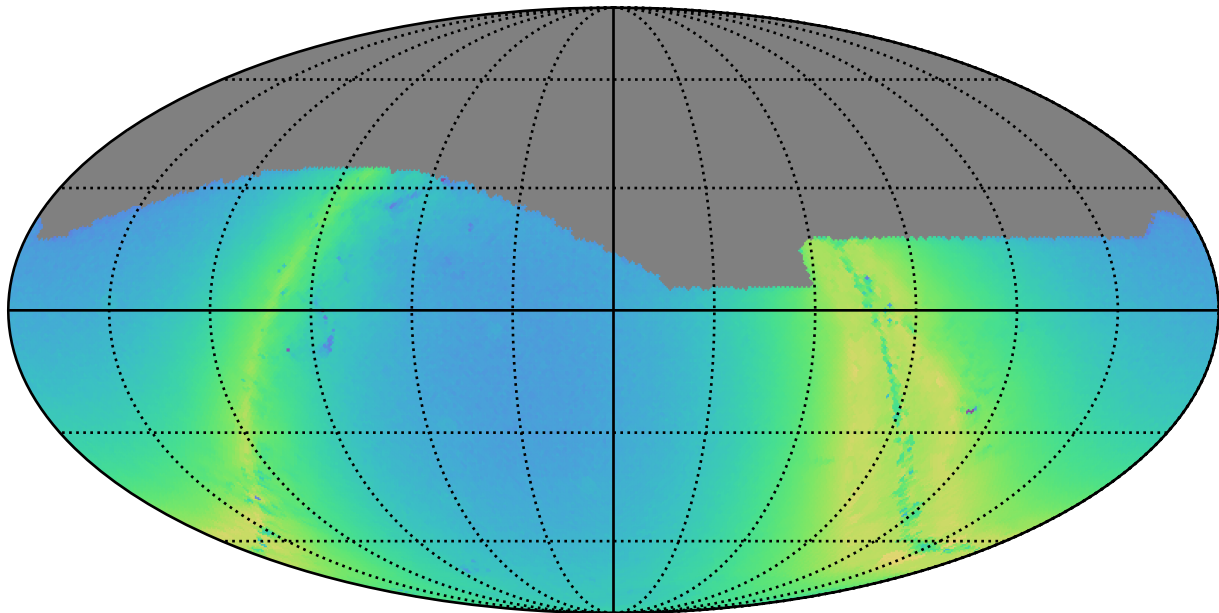
ddf_acor_sf15_lsf20_lsr20_v3.4_10yrs g: N stars to Precision 0.20
