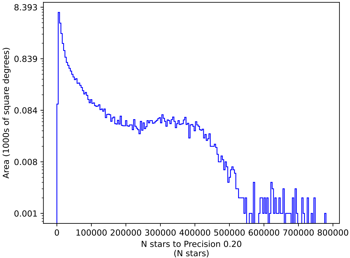
ddf_acor_sf15_lsf20_lsr20_v3.4_10yrs g: N stars to Precision 0.20
