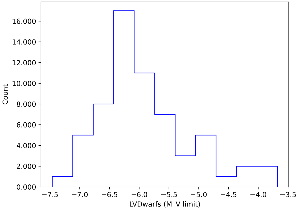
ddf_acor_sf15_lsf20_lsr20_v3.4_10yrs gi: LVDwarfs
