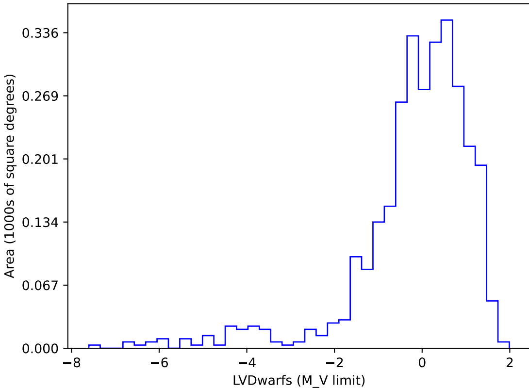
ddf_acor_sf15_lsf20_lsr20_v3.4_10yrs gi SCP: LVDwarfs
