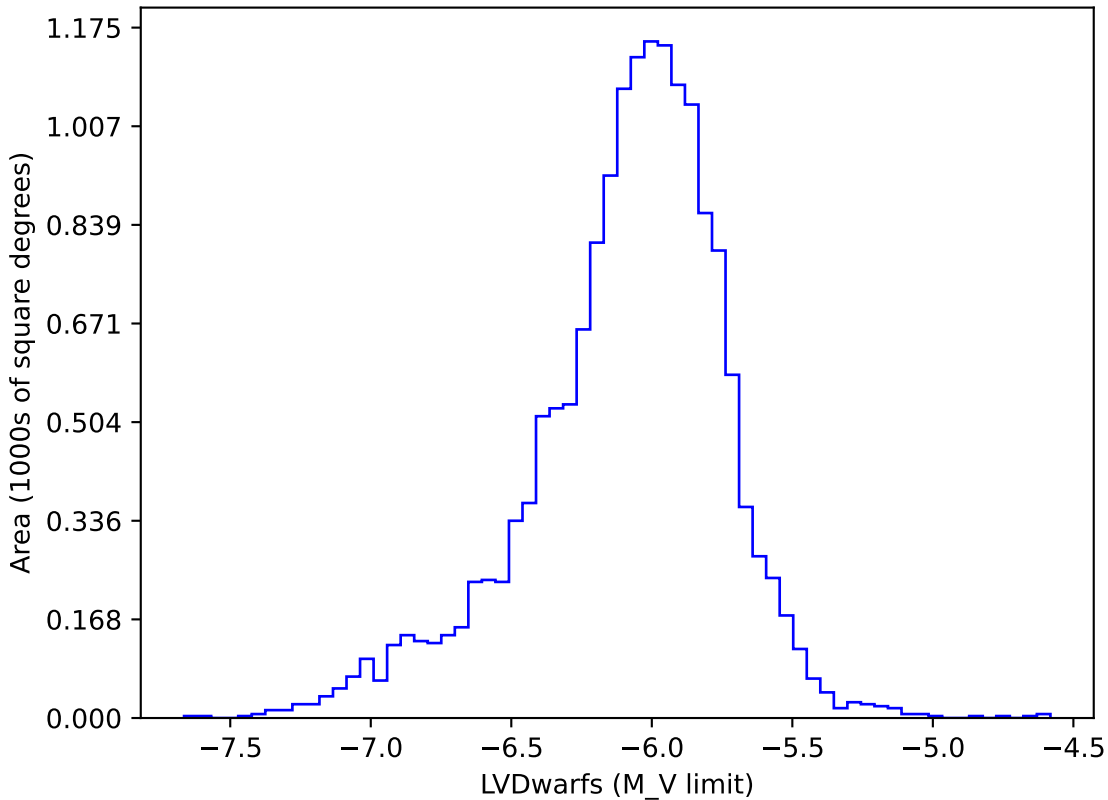
ddf_acor_sf15_lsf20_lsr20_v3.4_10yrs gi: LVDwarfs
