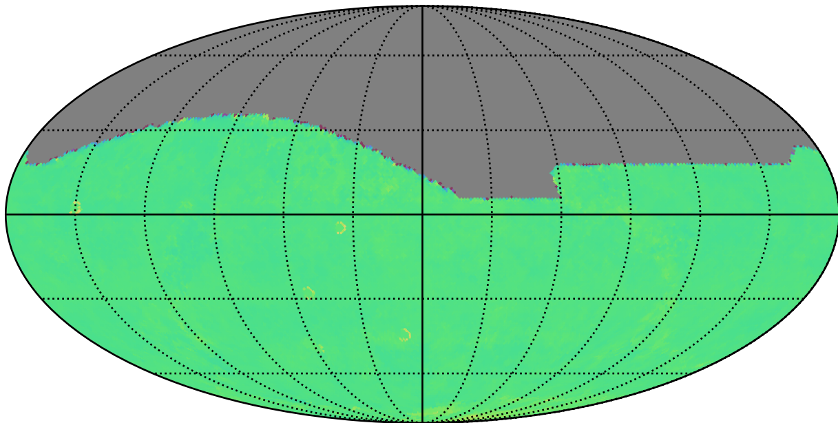
ddf_acor_sf15_lsf20_lsr20_v3.4_10yrs r: Kuiper rotTelPos
