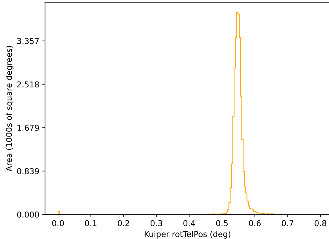
ddf_acor_sf15_lsf20_lsr20_v3.4_10yrs r: Kuiper rotTelPos
