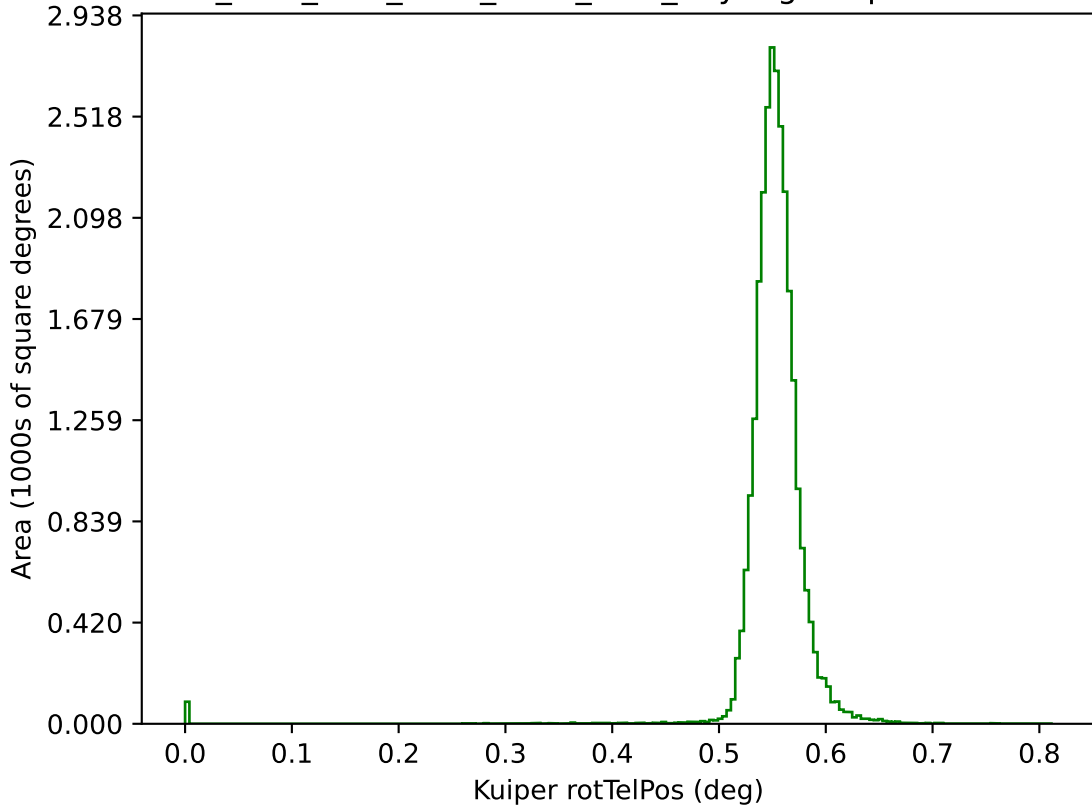
ddf_acor_sf15_ls20_lsr20_v3.4_10yrs g: Kuiper rotTelPos
