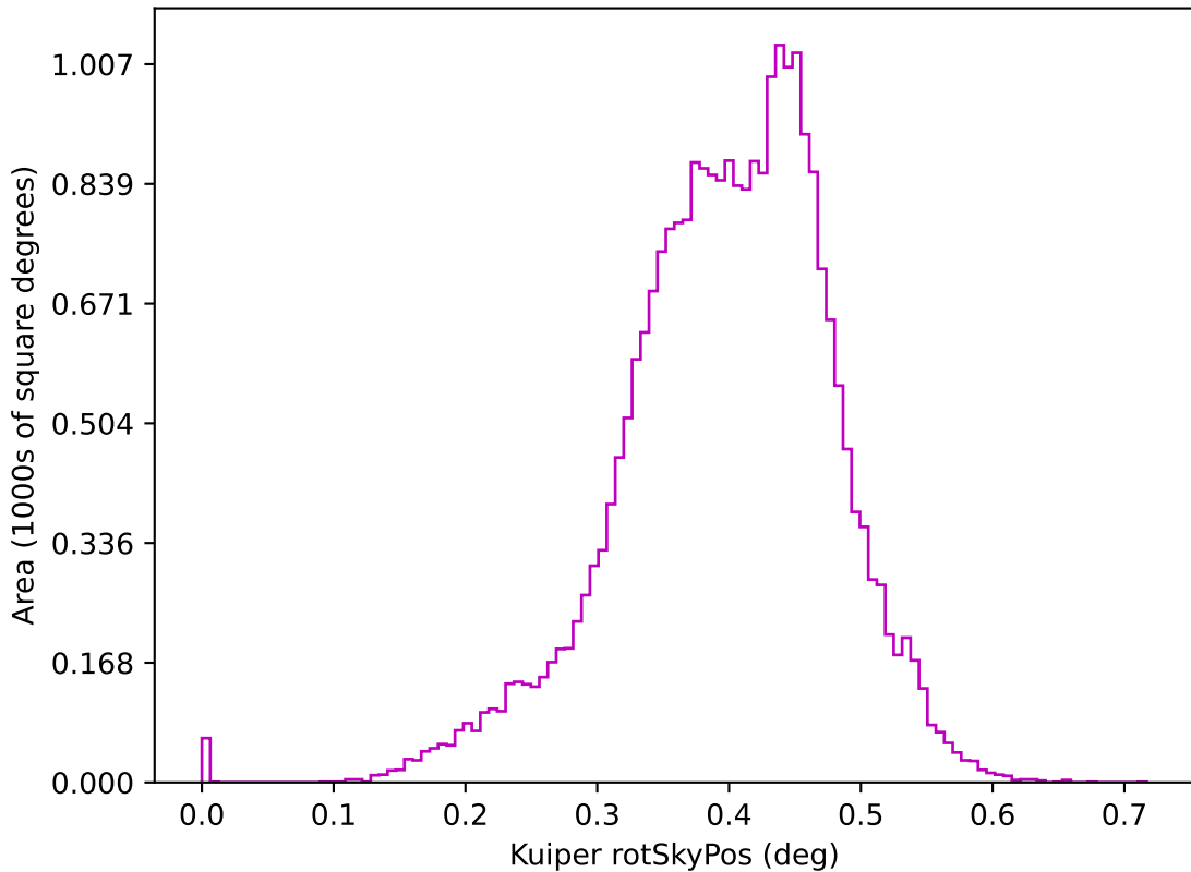
ddf_acor_sf15_lsf20_lsr20_v3.4_10yrs z: Kuiper rotSkyPos
