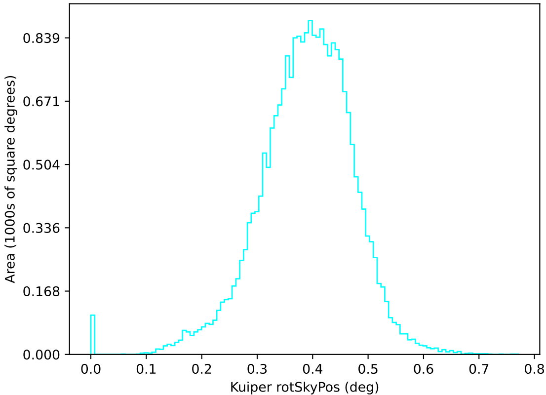
ddf_acor_sf15_ls20_lsr20_v3.4_10yrs u: Kuiper rotSkyPos
