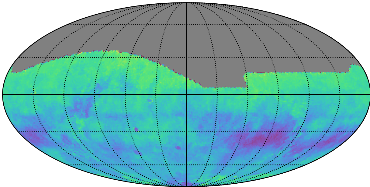
ddf_acor_sf15_lsf20_lsr20_v3.4_10yrs r: Kuiper rotSkyPos
