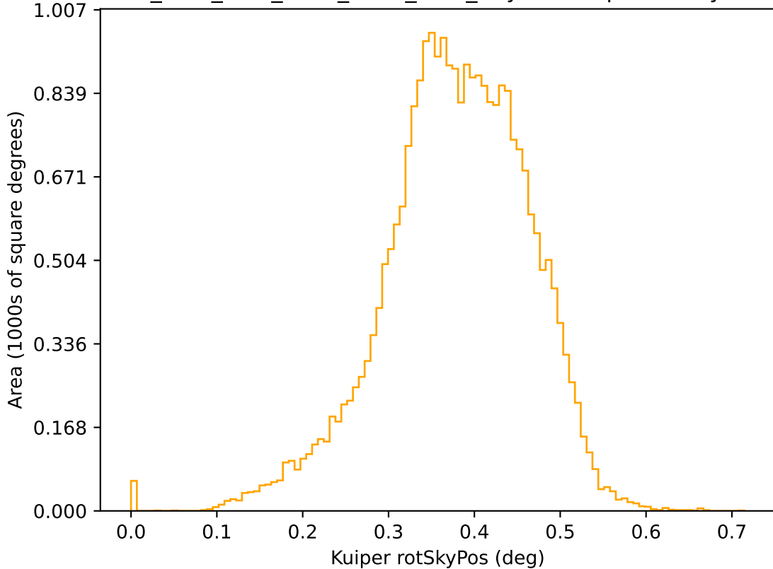
ddf_acor_sf15_ls20_lsr20_v3.4_10yrs r: Kuiper rotSkyPos
