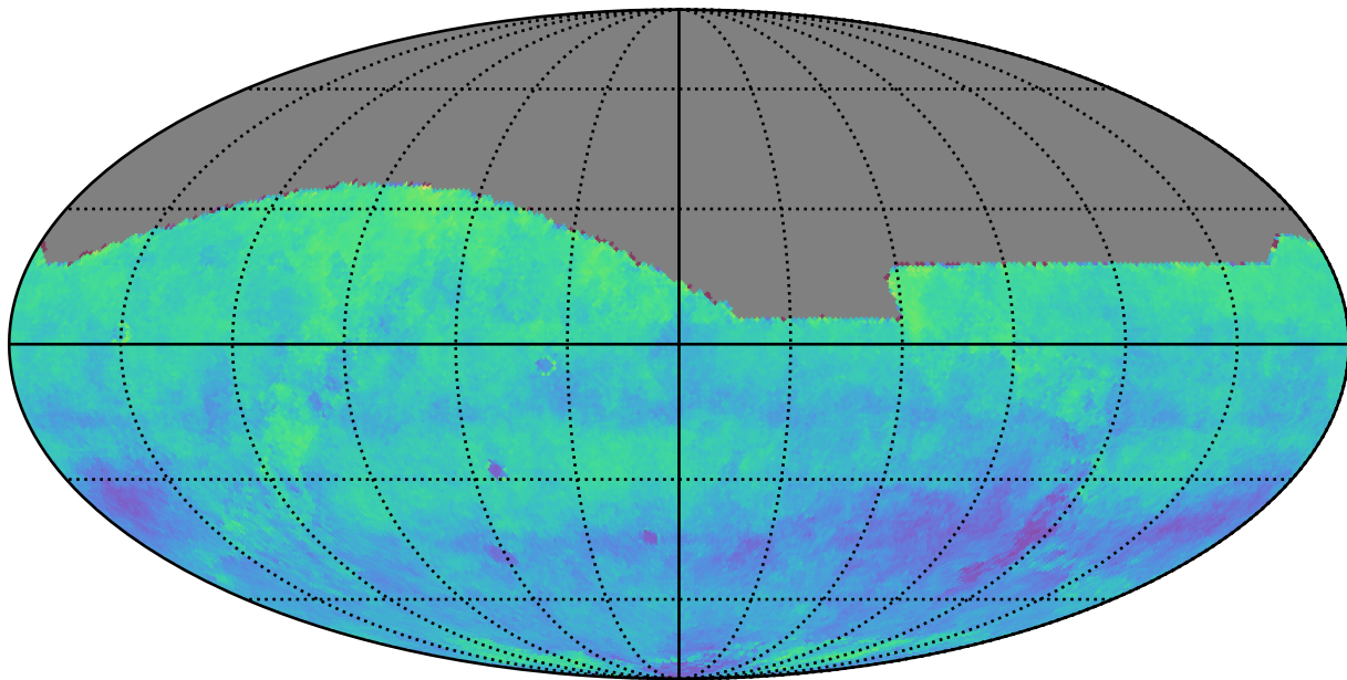
ddf_acor_sf15_lsf20_lsr20_v3.4_10yrs i: Kuiper rotSkyPos
