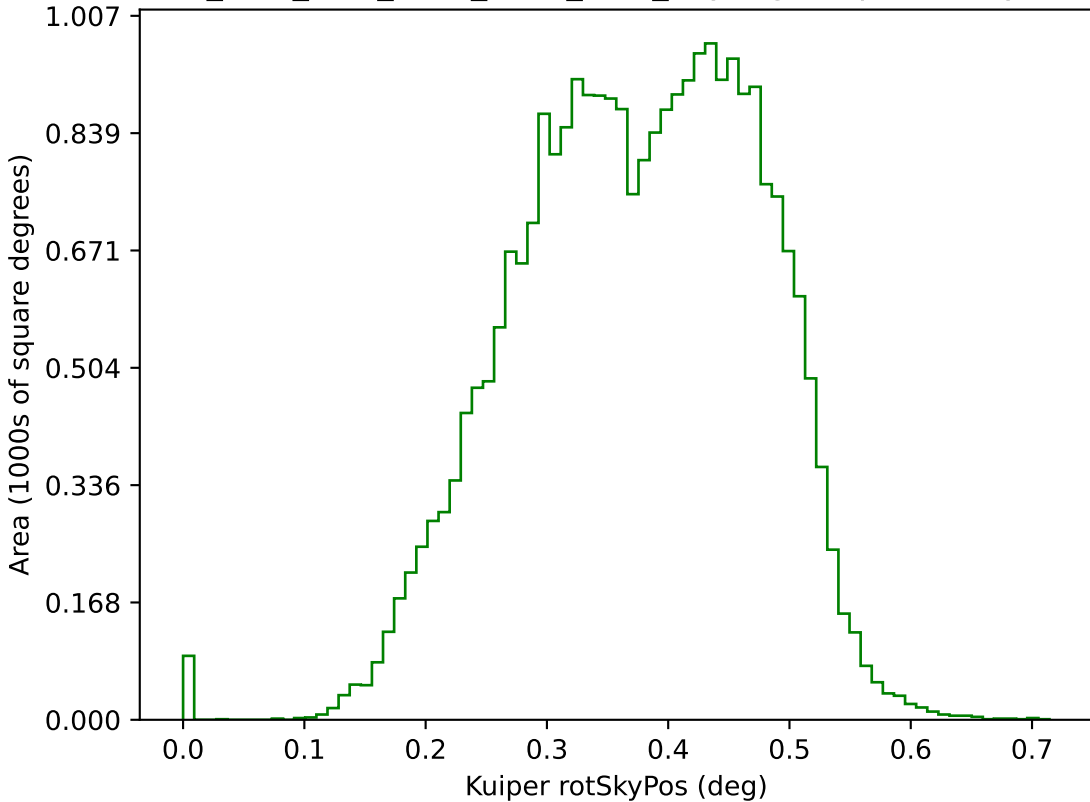
ddf_acor_sf15_lsf20_lsr20_v3.4_10yrs g: Kuiper rotSkyPos
