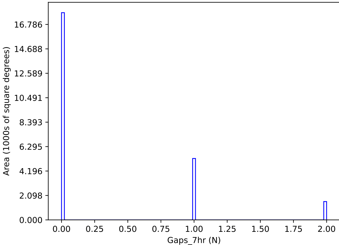
ddf_acor_sf15_lsf20_lsr20_v3.4_10yrs y band: Gaps_7hr
