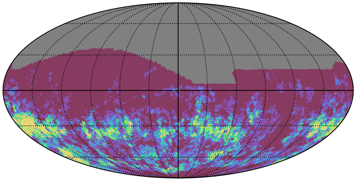
ddf_acor_sf15_lsf20_lsr20_v3.4_10yrs r band: Gaps_7hr
