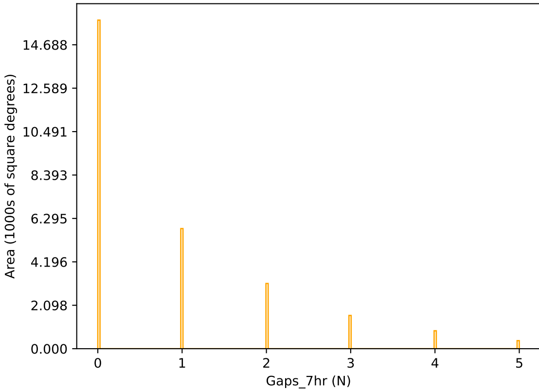
ddf_acor_sf15_lsf20_lsr20_v3.4_10yrs r band: Gaps_7hr
