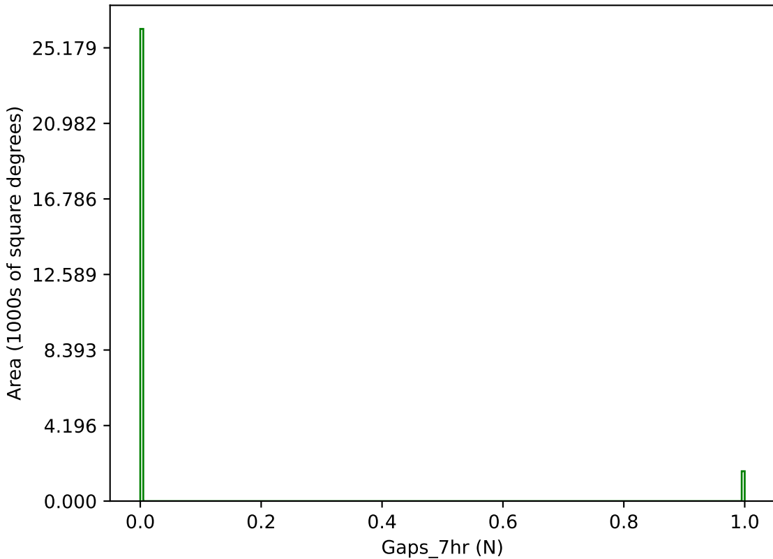
ddf_acor_sf15_lsf20_lsr20_v3.4_10yrs g band: Gaps_7hr
