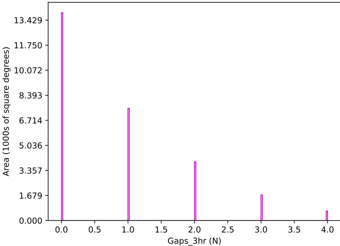
ddf_acor_sf15_lsf20_lsr20_v3.4_10yrs z band: Gaps_3hr
