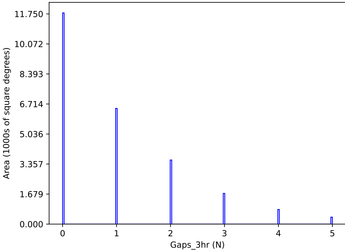
ddf_acor_sf15_ls20_lsr20_v3.4_10yrs y band: Gaps_3hr
