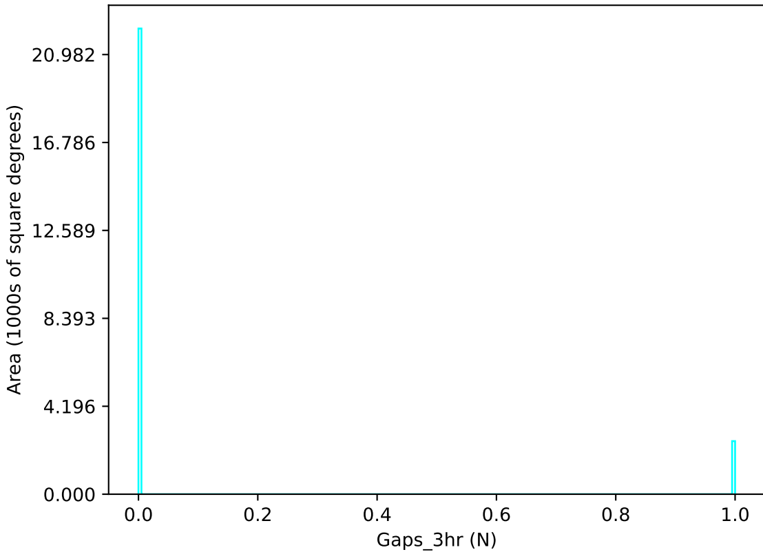
ddf_acor_sf15_lsf20_lsr20_v3.4_10yrs u band: Gaps_3hr
