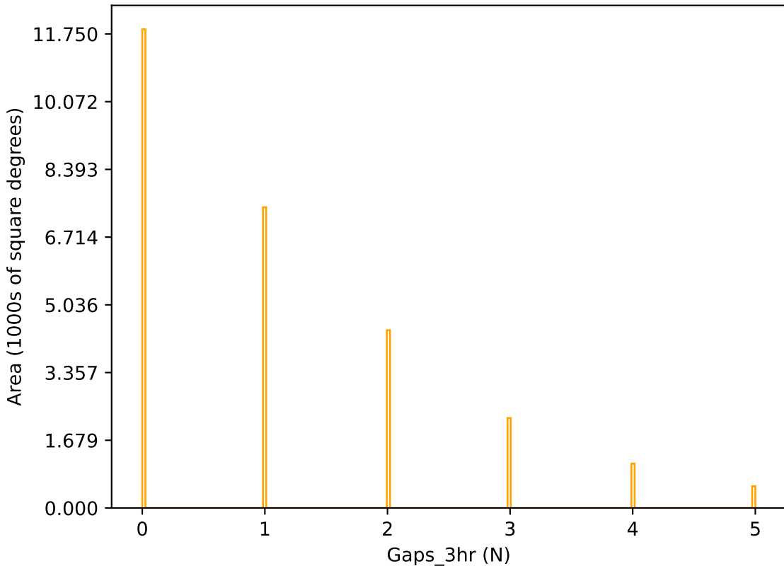
ddf_acor_sf15_lsf20_lsr20_v3.4_10yrs r band: Gaps_3hr
