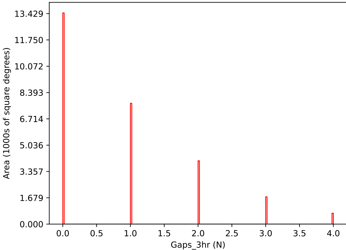
ddf_acor_sf15_lsf20_lsr20_v3.4_10yrs i band: Gaps_3hr
