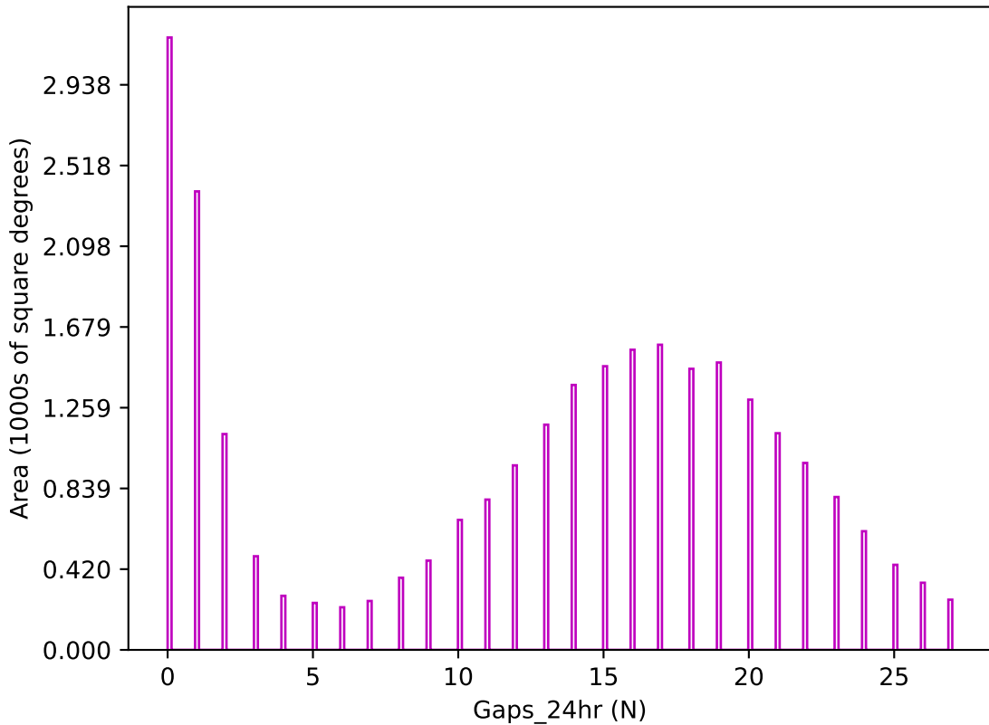
ddf_acor_sf15_lsf20_lsr20_v3.4_10yrs z band: Gaps_24hr
