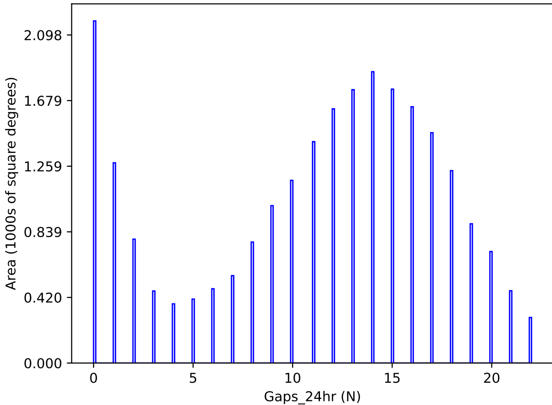
ddf_acor_sf15_lsf20_lsr20_v3.4_10yrs y band: Gaps_24hr
