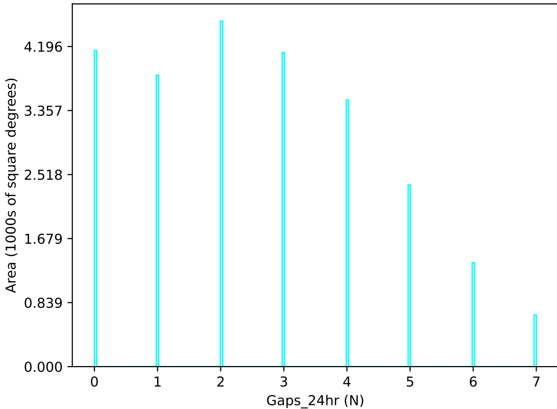
ddf_acor_sf15_lsf20_lsr20_v3.4_10yrs u band: Gaps_24hr
