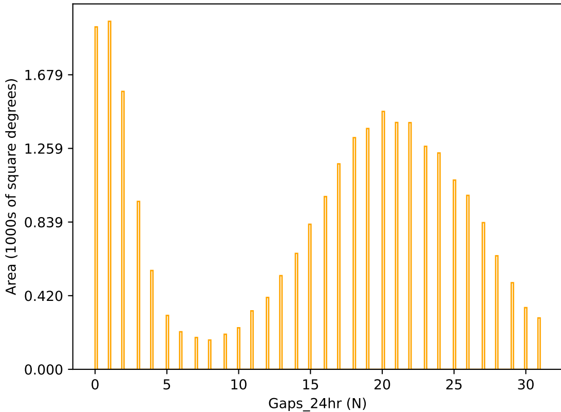
ddf_acor_sf15_ls20_lsr20_v3.4_10yrs r band: Gaps_24hr
