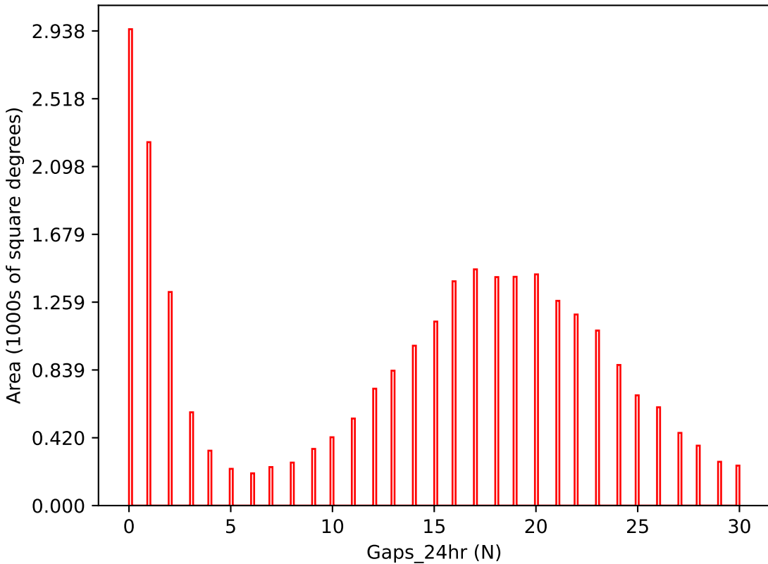
ddf_acor_sf15_lsf20_lsr20_v3.4_10yrs i band: Gaps_24hr
