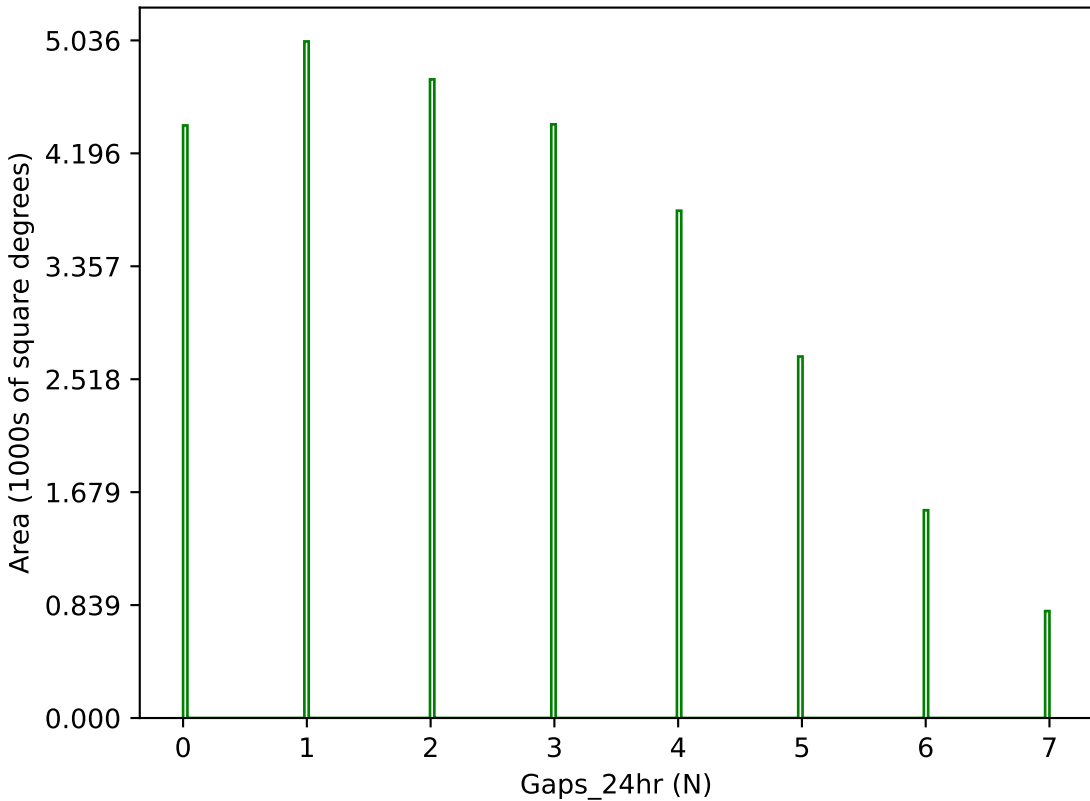
ddf_acor_sf15_lsf20_lsr20_v3.4_10yrs g band: Gaps_24hr
